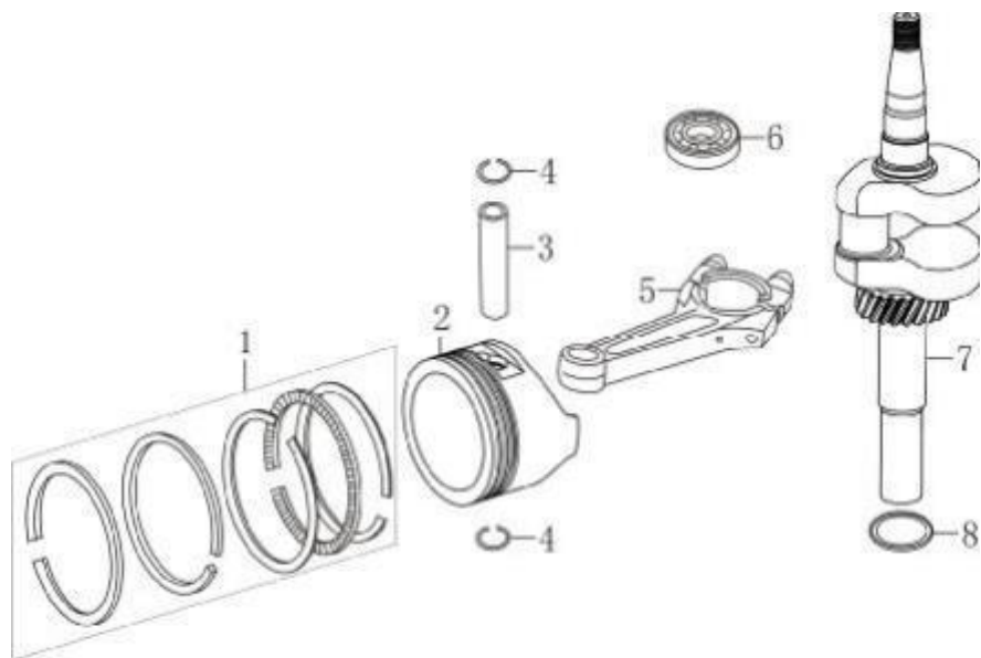
(Crankshaft/Piston/connecting rod)
