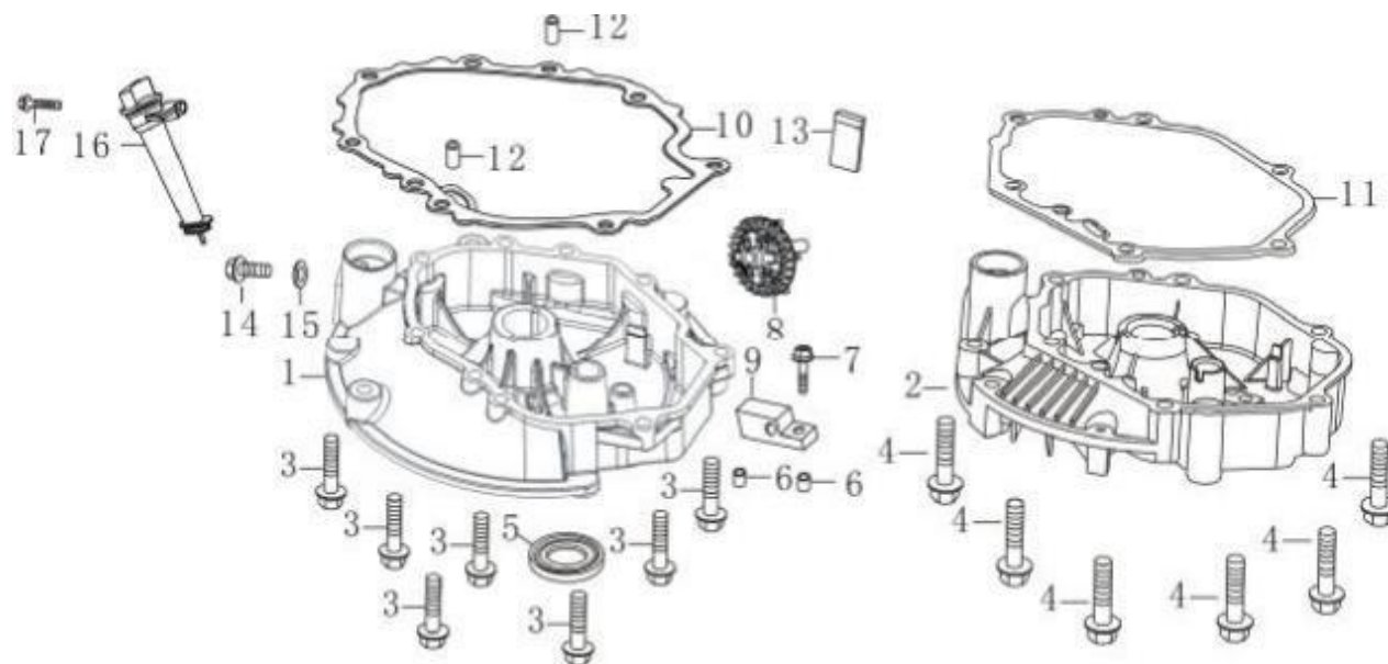
(Crankcase cover)
