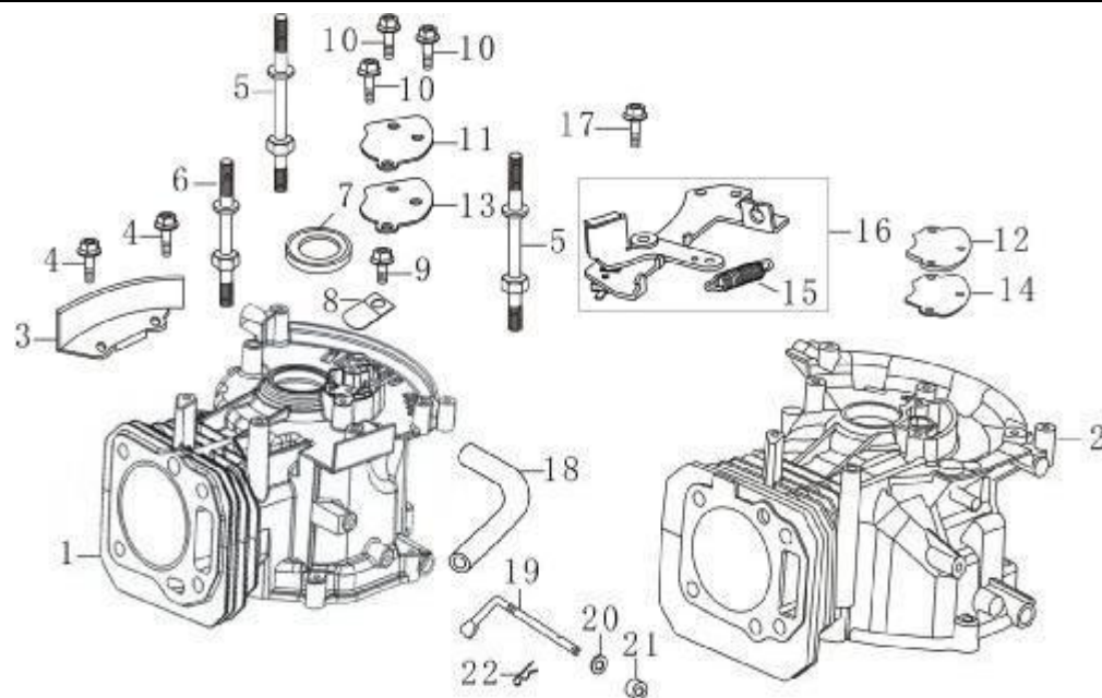
(Crankcase)
