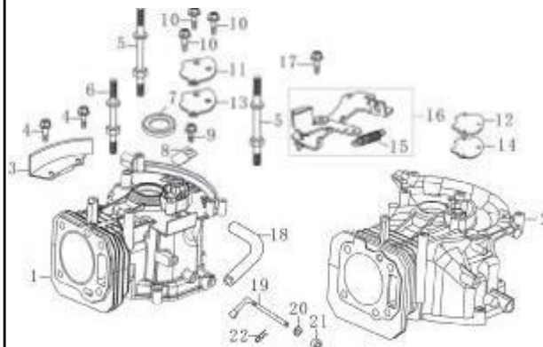
(Crankcase)
