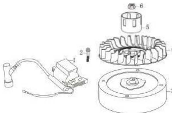
(Flywheel/Ignition Comp)
