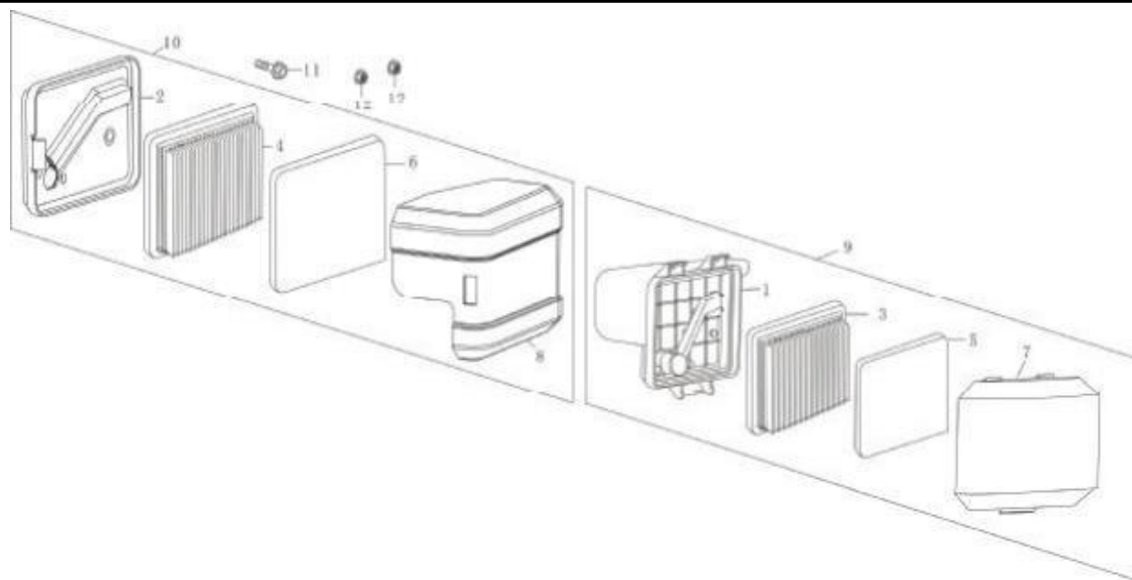
( Air cleaner )
